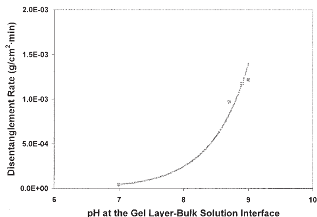
Figure 15. Effect of the interfacial pH on the disentanglement rate.
