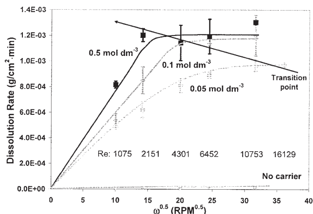
Figure 14. Change of the rate-limiting step ( \text{NH}_3 carrier).
