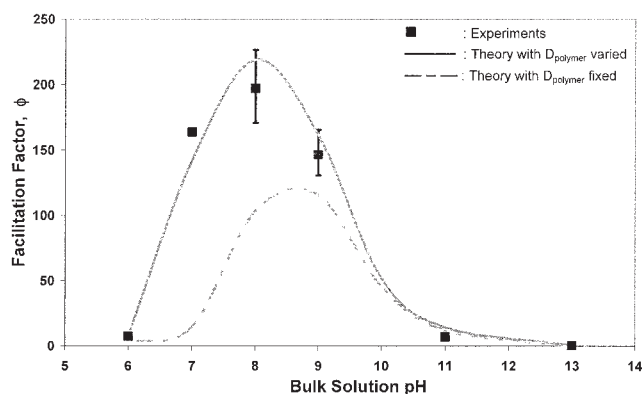
Figure 10. Effect of bulk solution pH on the facilitation factor ([NH 3 ] = 0.5 mol/L, pK a = 9.1).
