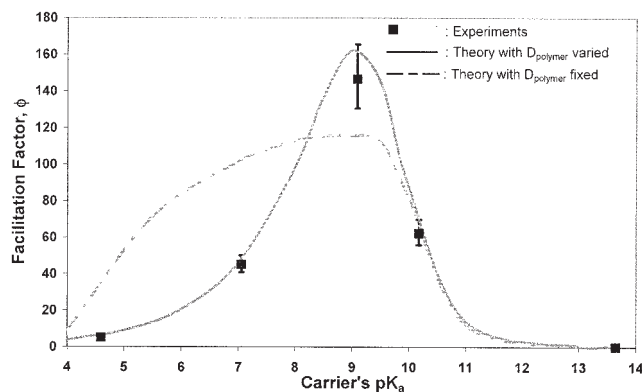
Figure 11. Effect of carrier's acidity on the facilitation factor ([carrier] = 0.5 mol/L, pH = 9).
